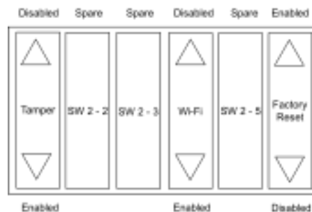
ACS300 SW-2 Switch Settings
