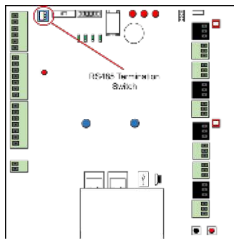
RS-485 Termination Switch Location
